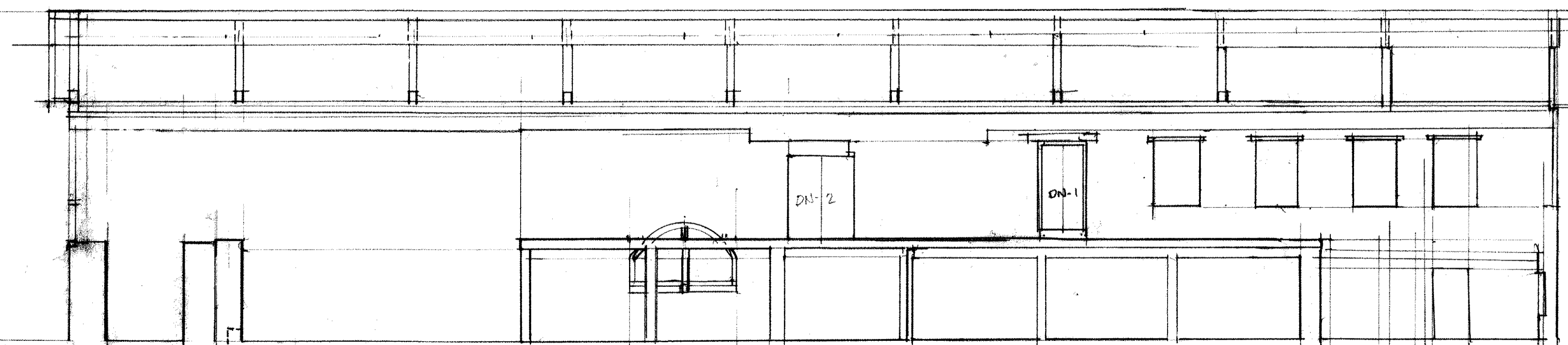
SECTION LOOKING NORTH 1/8"
